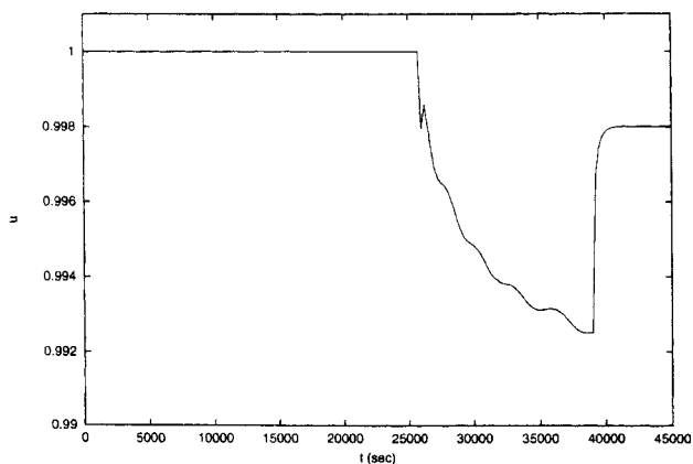
Figure 10. Manipulated input profile-PI controller.
