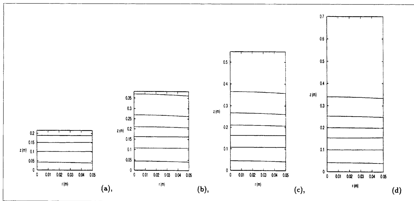
Figure 4. Temperature of crystal as a function of radial and axial coordinates for T_{amb} = 1,000 K.
