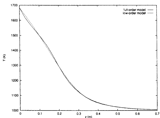
Figure 13. Comparison of temperature profiles of open loop system at T_{\text{amb}} = 600 K between the 2-D model at r = 0.05 m and the reduced-order model at the end of the process.
