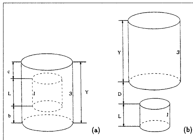
Figure A3. Cylinder to cylinder view factors.
