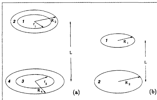
Figure A1. View factors.
